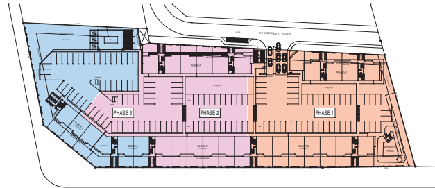
PHASING PLAN
